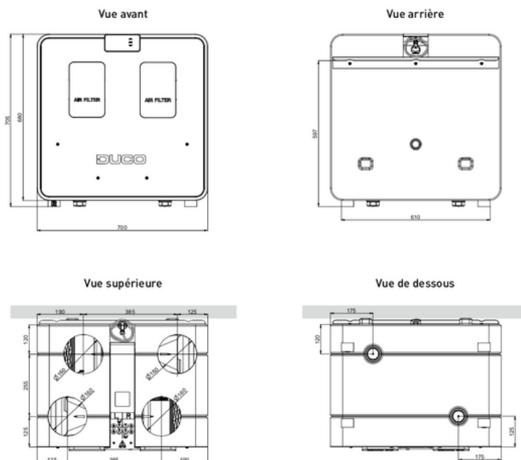
Dimensions de la DucoBox Energy Comfort
